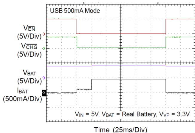
Charger On/Off Control from \overline{\text{EN}}
