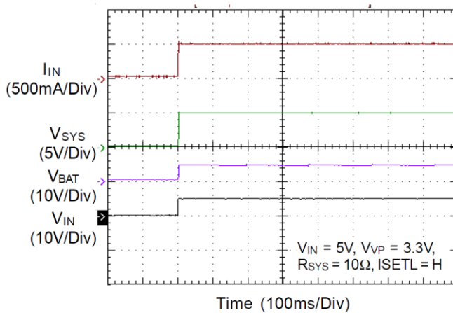
V_{\text{IN}} Hot-plug without NVC/Battery
