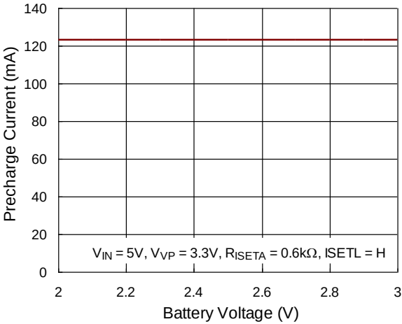
Precharge Current vs. Battery Voltage
