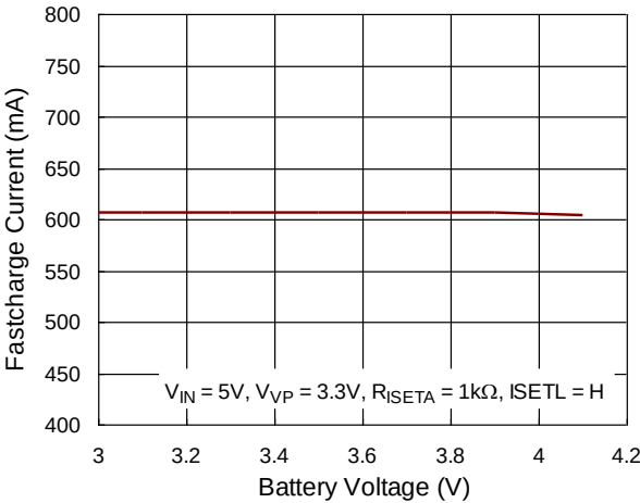
Fastcharge Current vs. Battery Voltage
