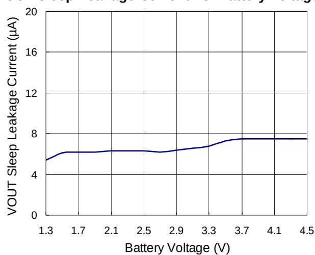
VOUT Sleep Leakage Current vs. Battery Voltage
