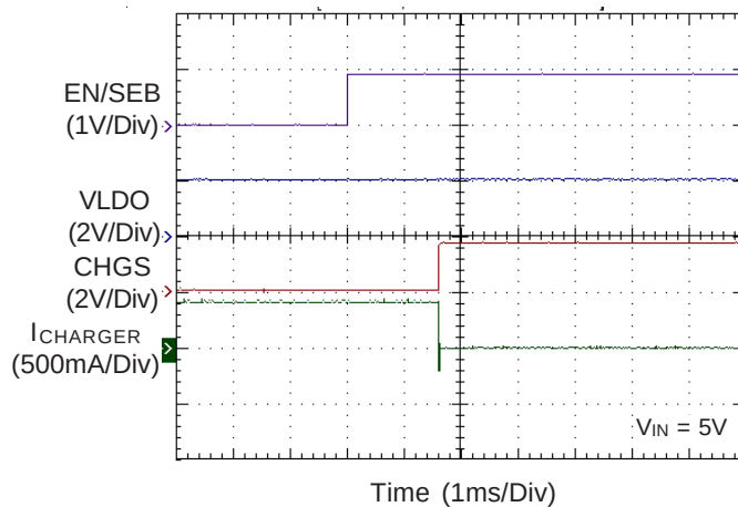
EN/SET Shut-Down
