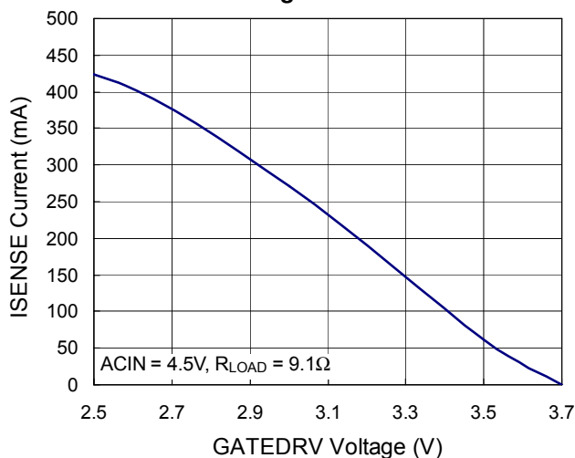
GATEDRV Voltage vs. ISENSE Current
