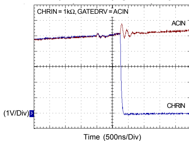
Input OVP Propagation Delay
