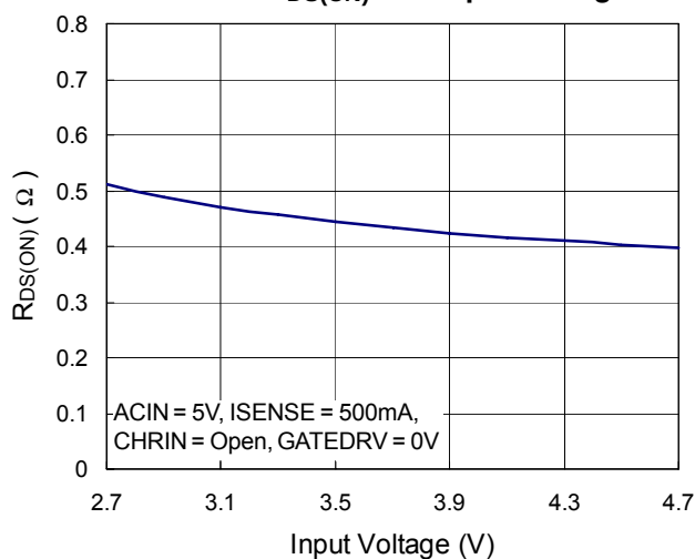
ISENSE R DS(ON) vs. Input Voltage
