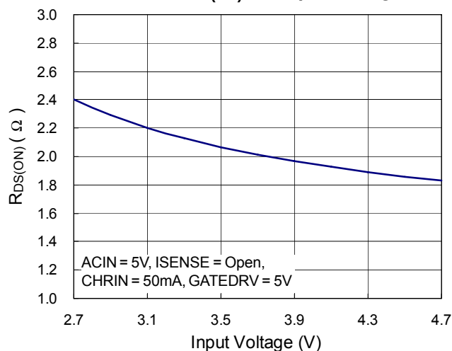
CH RIN R DS(ON) vs. Input Voltage
