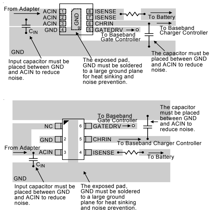
Figure 4. PCB Layout Guide
