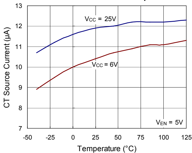
CT Source Current vs. Temperature
