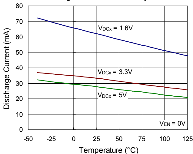
Discharge Current vs. Temperature
