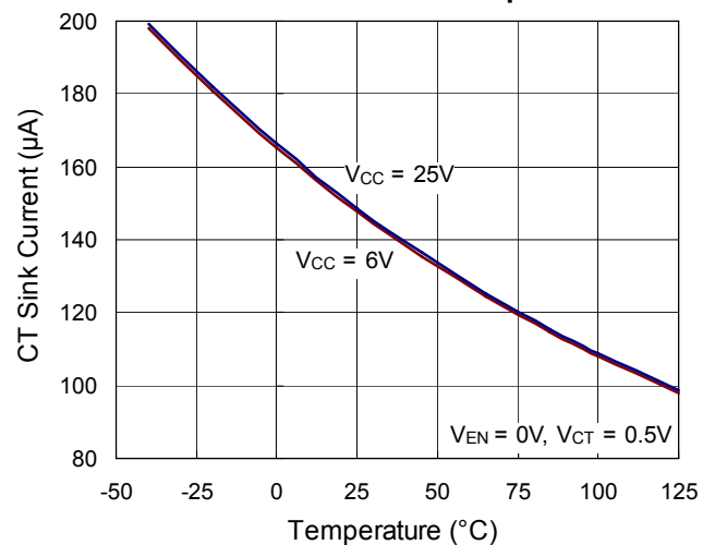
CT Sink Current vs. Temperature
