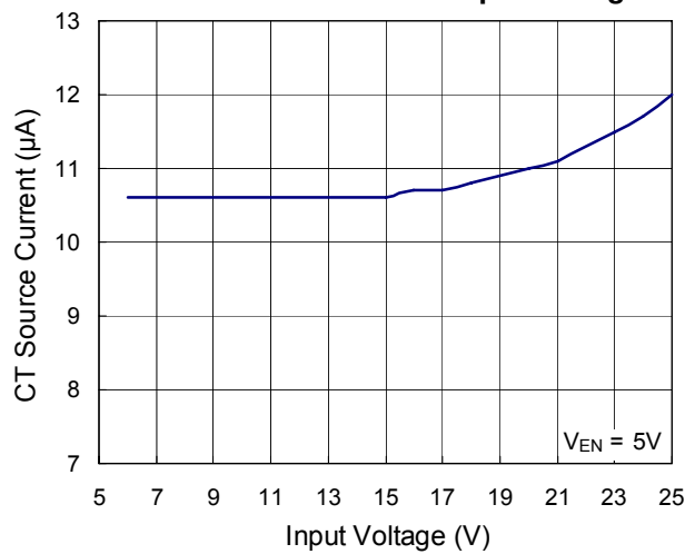
CT Source Current vs. Input Voltage
