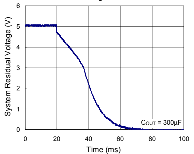
VDCx Discharge Characteristic
