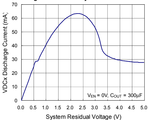
Discharge Current vs. System Residual Voltage
