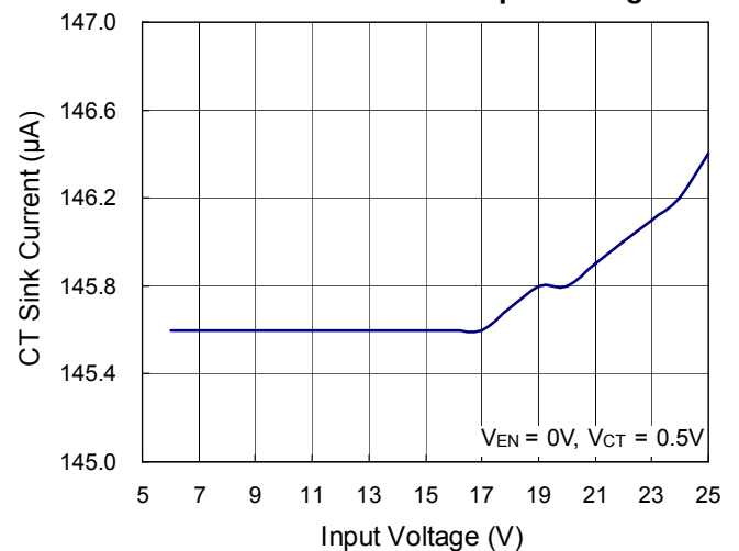
CT Sink Current vs. Input Voltage
