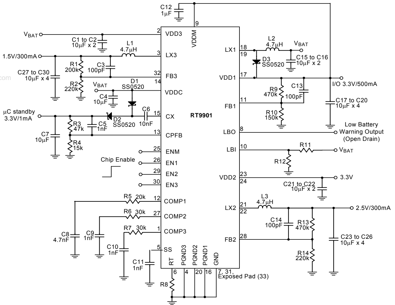
Figure 2. Typical Application Circuit from 2-AA Battery Supply
