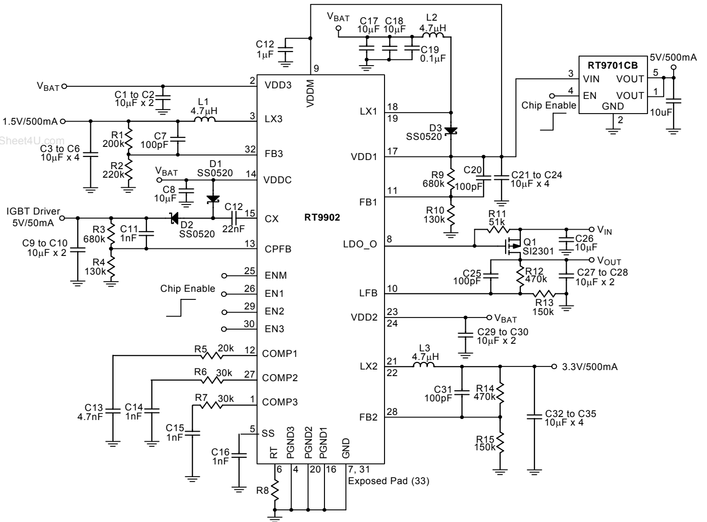
Figure 2. Typical Application Circuit from 1-cell Li+ Battery
