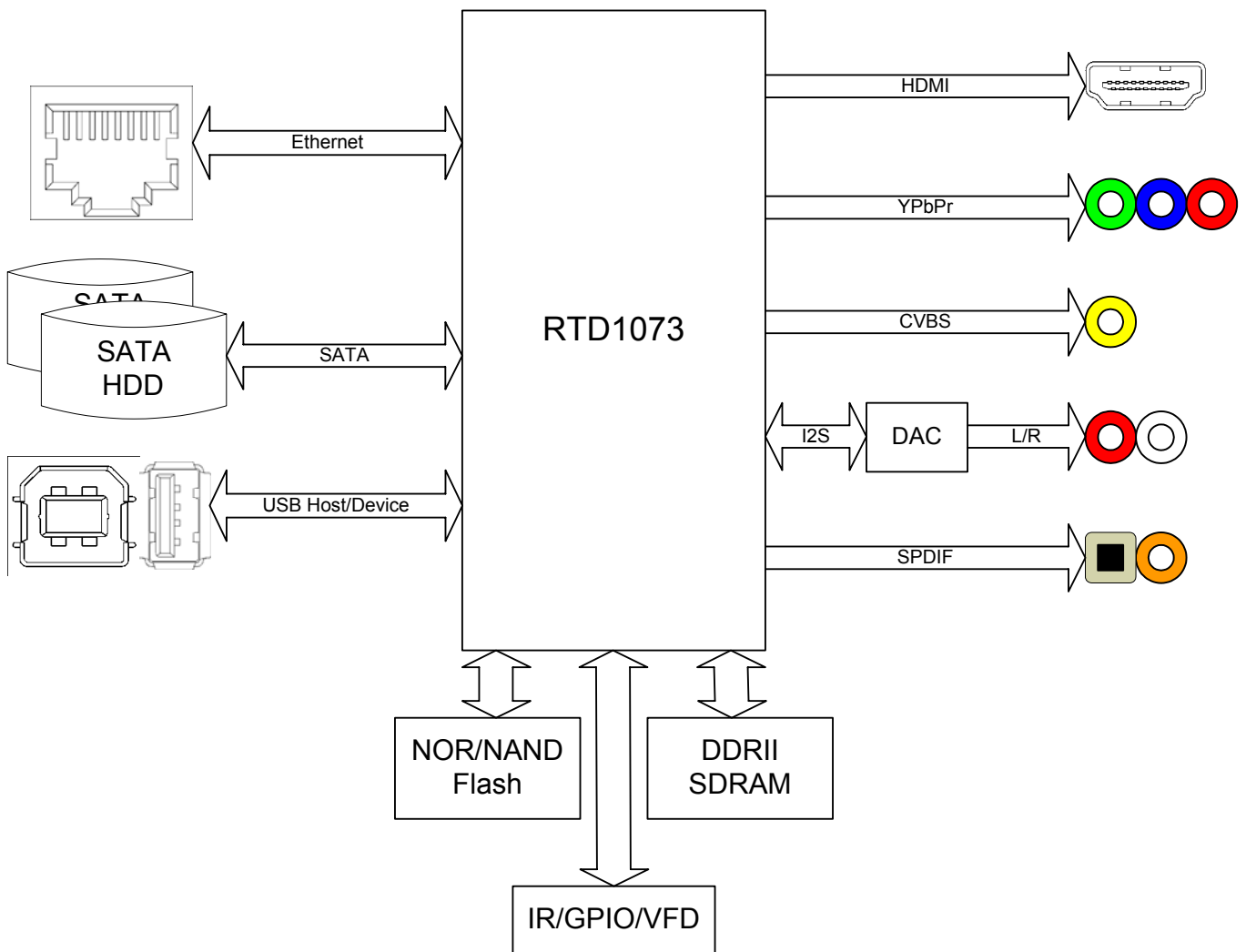
Figure 1. Application Diagram
