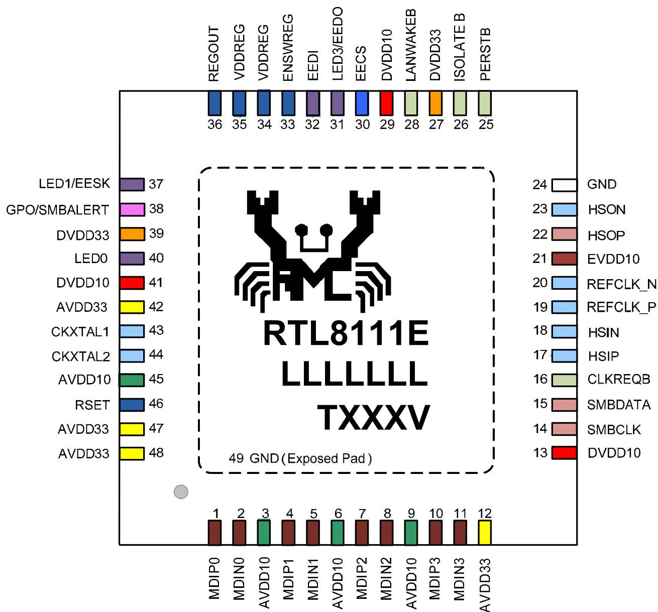
Figure 1. Pin Assignments
