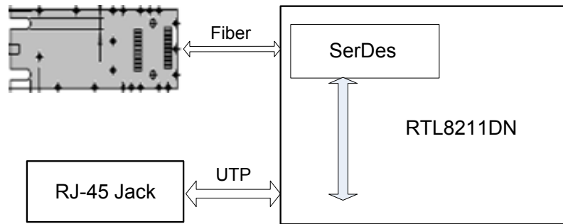
Figure 3. Fiber to UTP (Bridge Mode) Application Diagram
