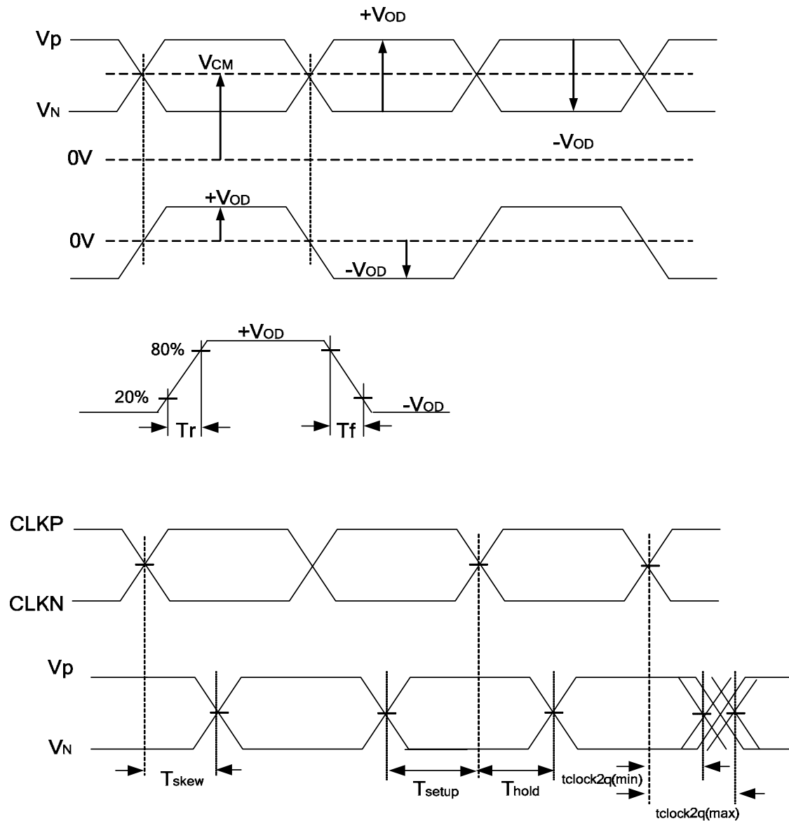
Figure 28. SGMII Timing Modes
