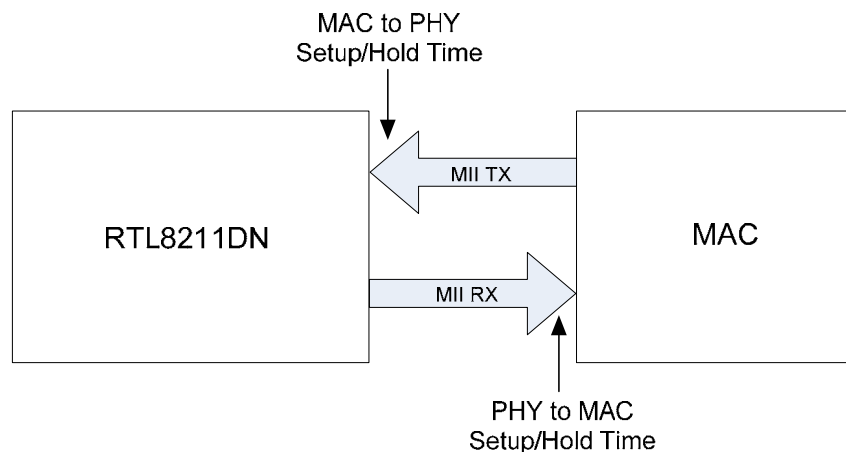
Figure 23. MII Interfaces Setup/Hold Time Definitions
