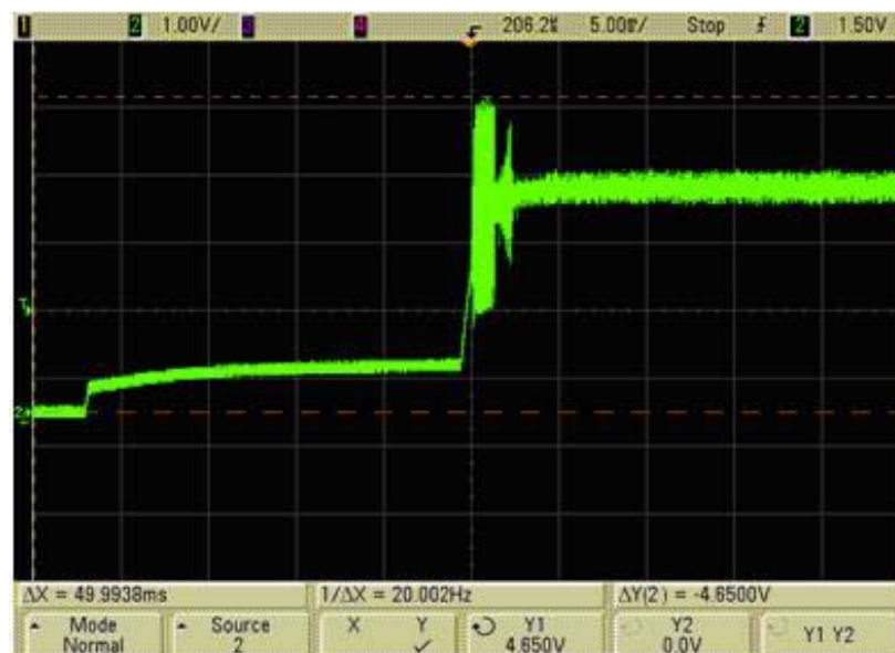
Figure 13. Input Voltage Overshoot >4V (Bad)
