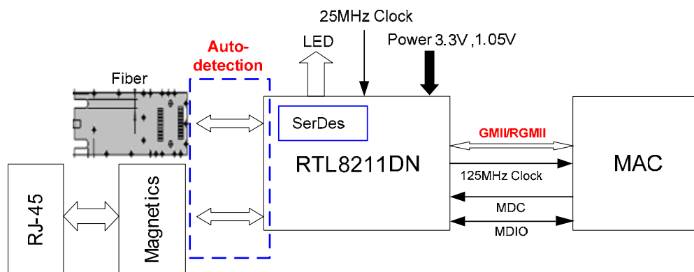
Figure 5. UTP/Fiber Auto-Detection to GMII/RGMII Application Diagram
