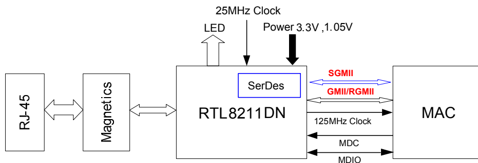
Figure 2. UTP Application Diagram
