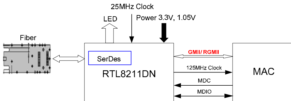
Figure 1. Fiber Application Diagram
