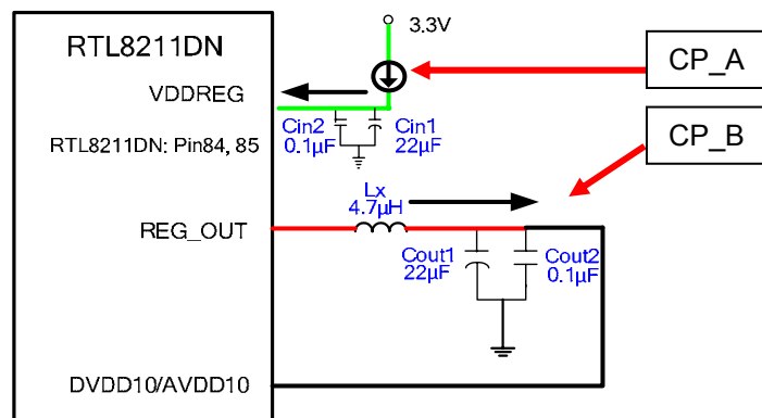
Figure 19. Switching Regulator Efficiency Measurement Checkpoint
