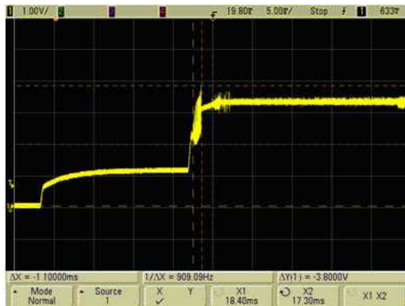
Figure 12. Input Voltage Overshoot <4V (Good)
