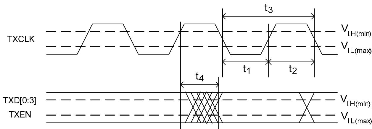
Figure 24. MII Transmission Cycle Timing
