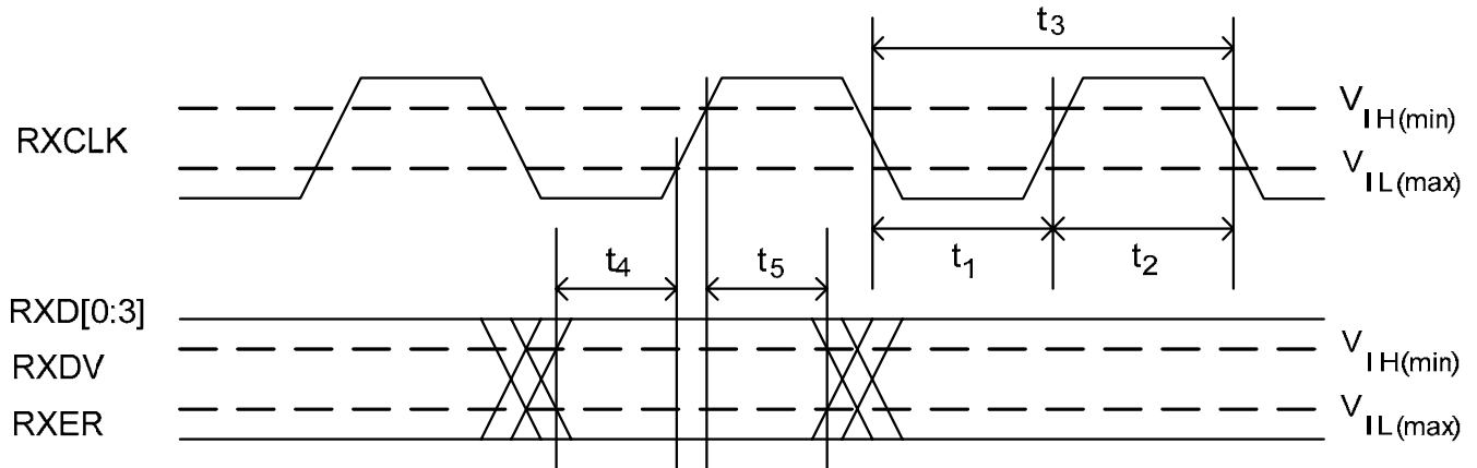
Figure 25. MII Reception Cycle Timing
