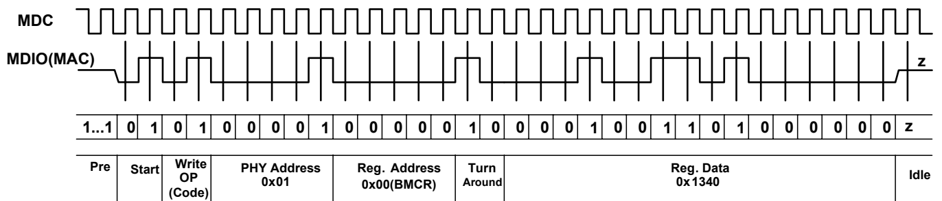
Figure 10. MDC/MDIO Write Timing
