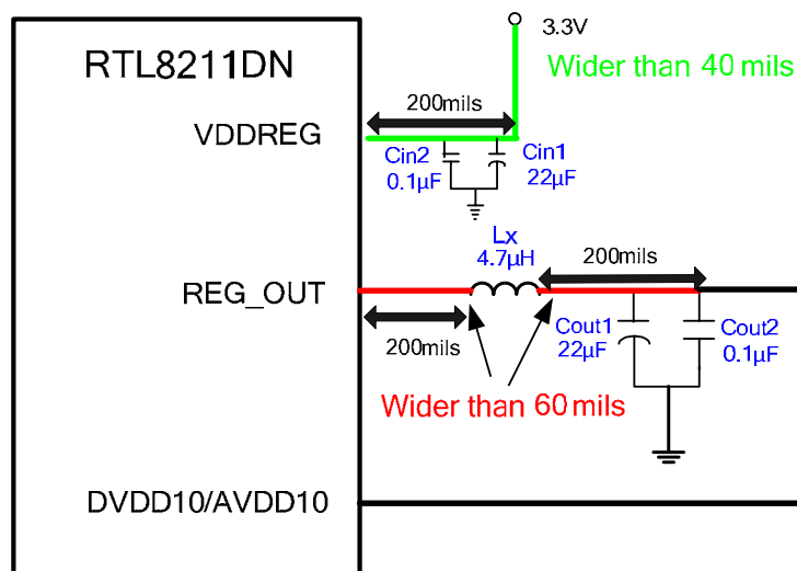
Figure 11. Switching Regulator
