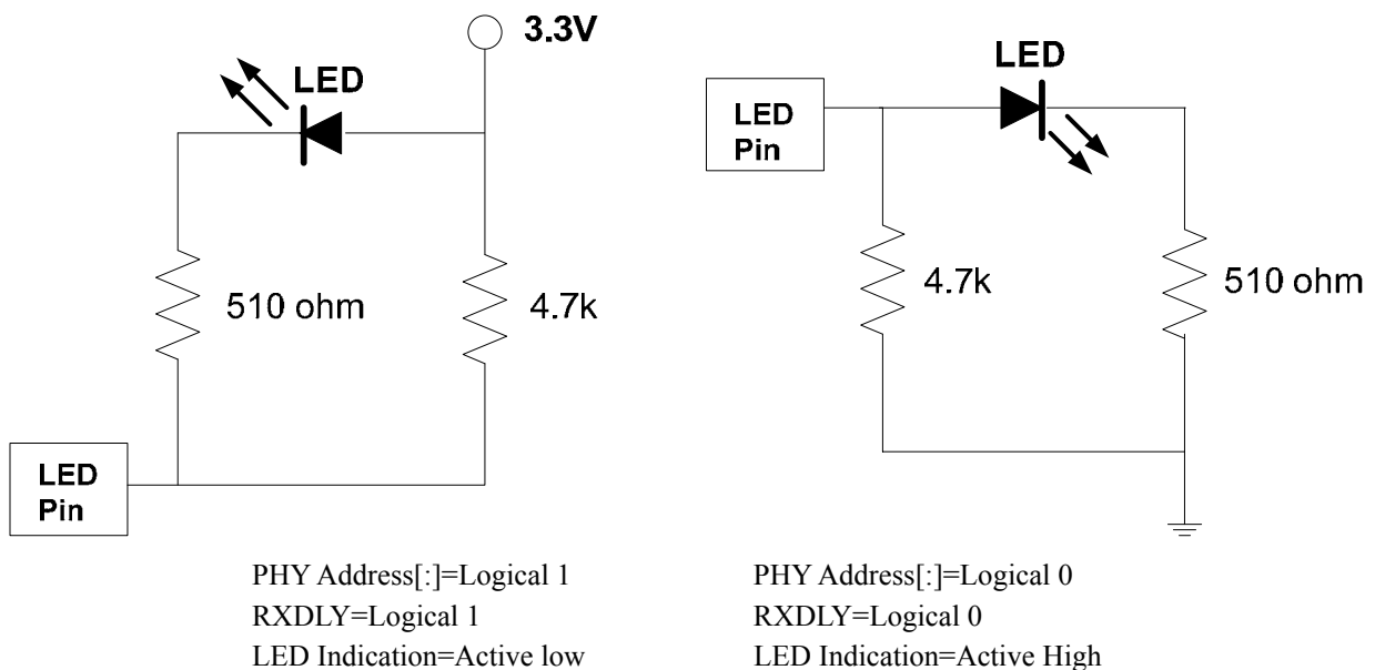
Figure 8. LED and PHY Address Configuration
