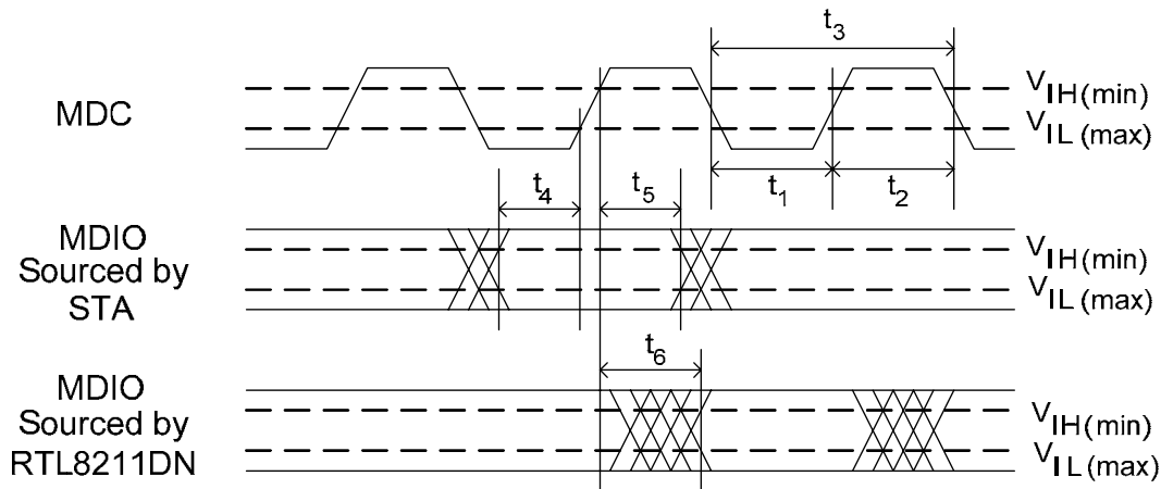
Figure 22. MDC/MDIO Timing
