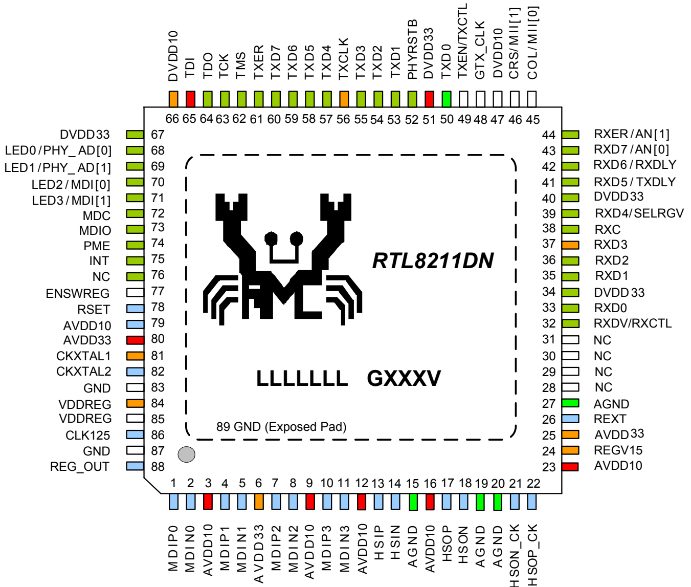
Figure 6. Pin Assignments
