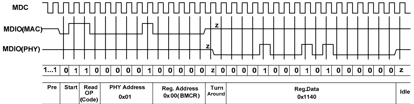
Figure 9. MDC/MDIO Read Timing
