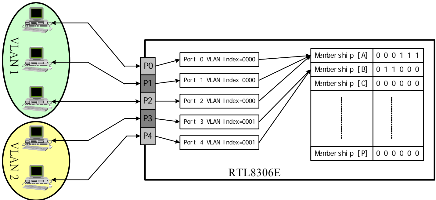
Figure 14. VLAN Grouping Example
