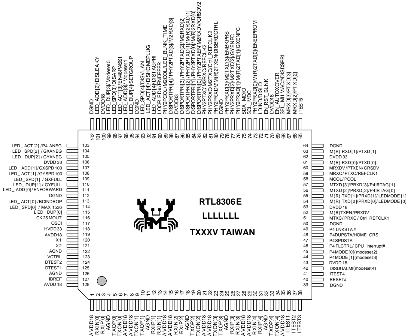
Figure 2. Pin Assignments
