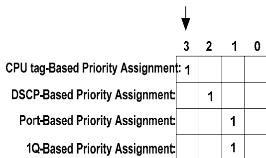
Figure 19. Packet Priority Selection
