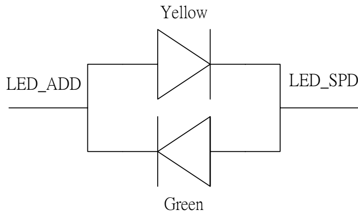
Figure 27. Two-Pin Bi-Color LED for SPD Pull-Down
