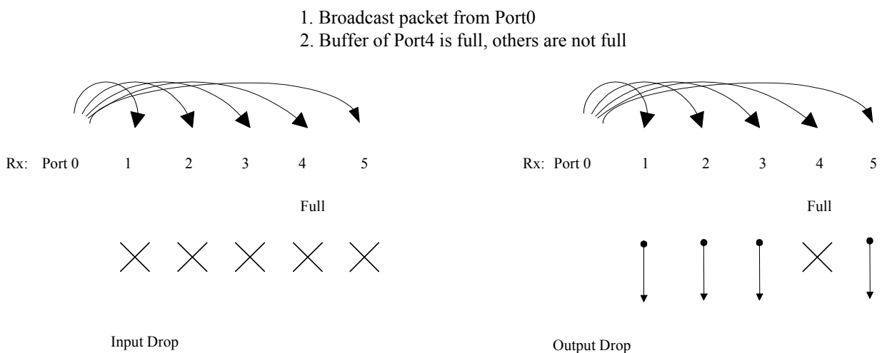
Figure 23. Broadcast Input Drop vs. Output Drop
