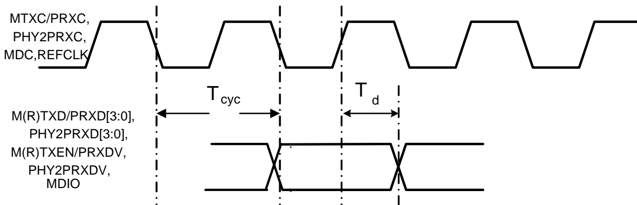
Figure 29. Transmission Data Timing of MII/RMII/SMI Interface
