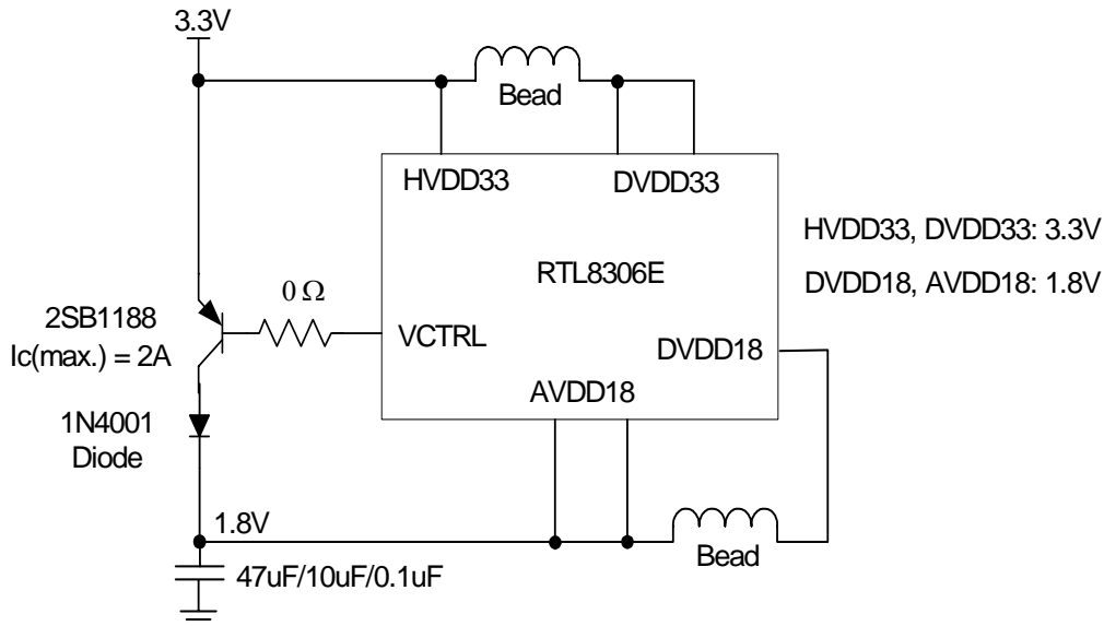
Figure 13. Using a PNP Transistor to Transform 3.3V Into 1.8V
