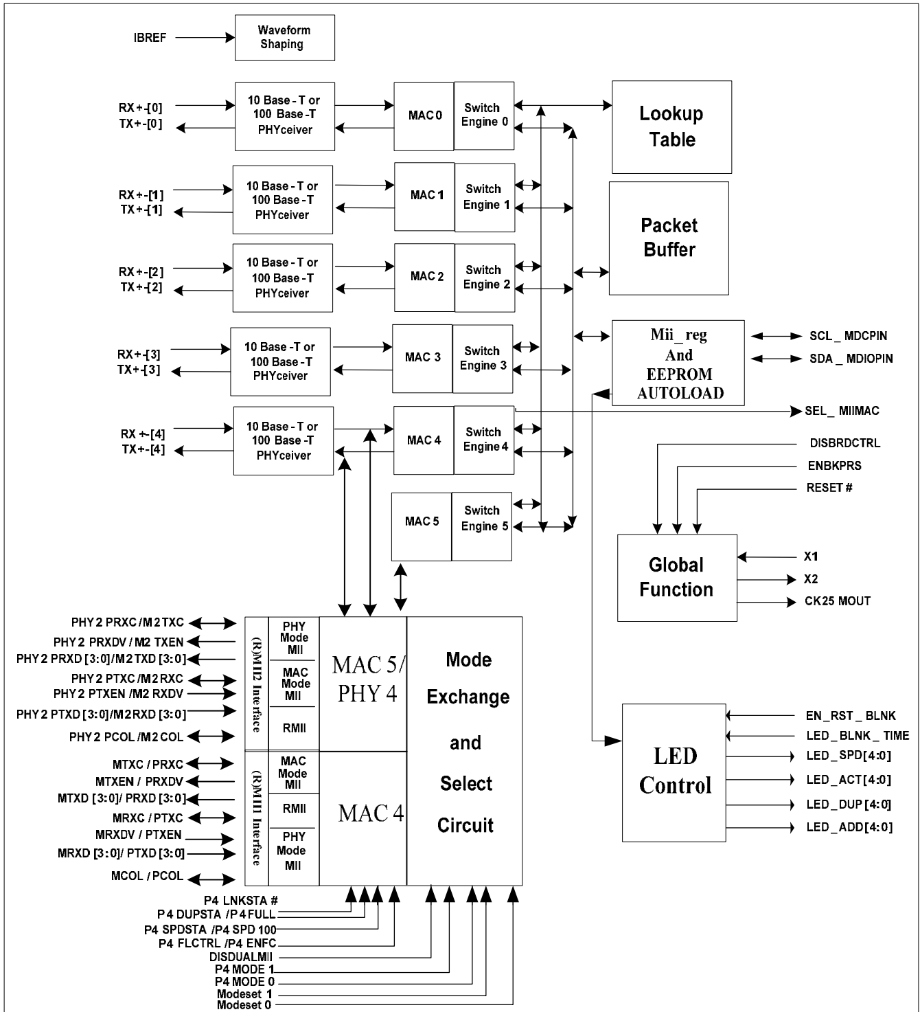
Figure 1. Block Diagram
