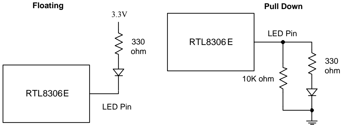
Figure 25. Floating and Pull-Down of LED Pins for Single-Color LED
