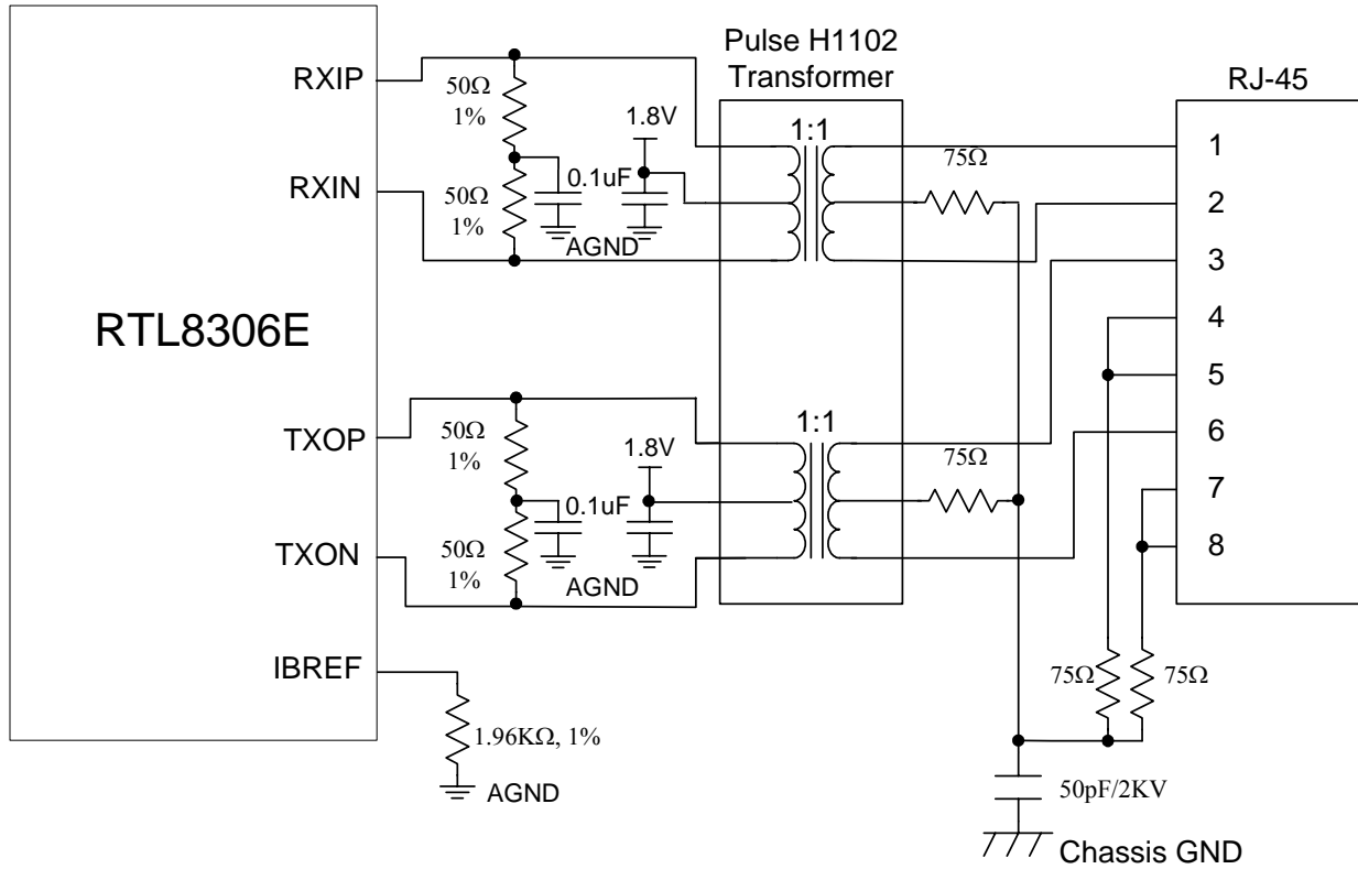
Figure 31. UTP Application for Transformer with Separate Central Tap
