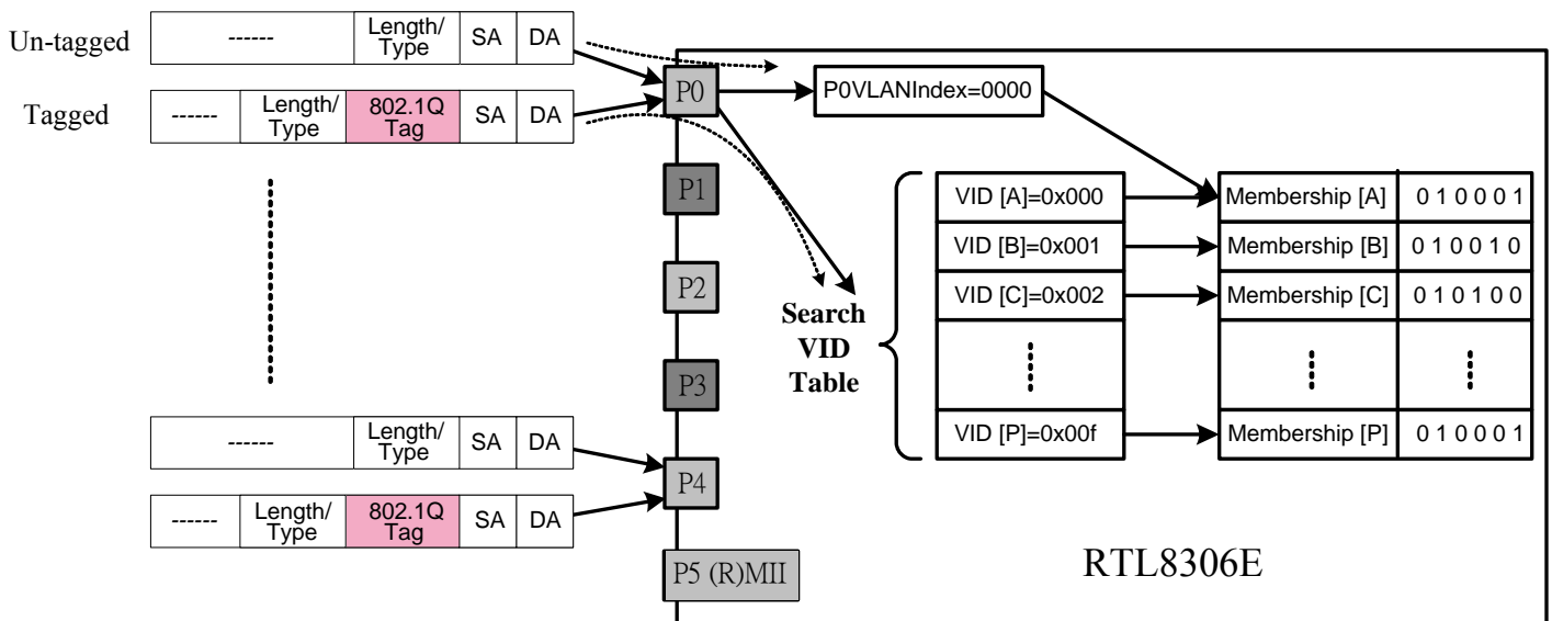
Figure 16. Tagged and Untagged Packet Forwarding when 802.1Q Tag Aware VLAN is Enabled
