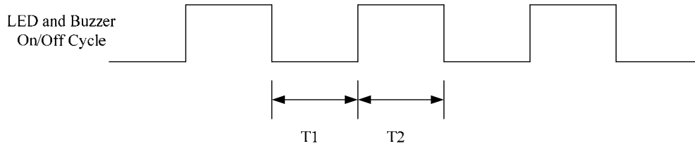
Figure 10. LED and Buzzer Control Signal for Loop Detection
