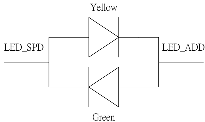
Figure 26. Two-Pin Bi-Color LED for SPD Floating or Pull-high
