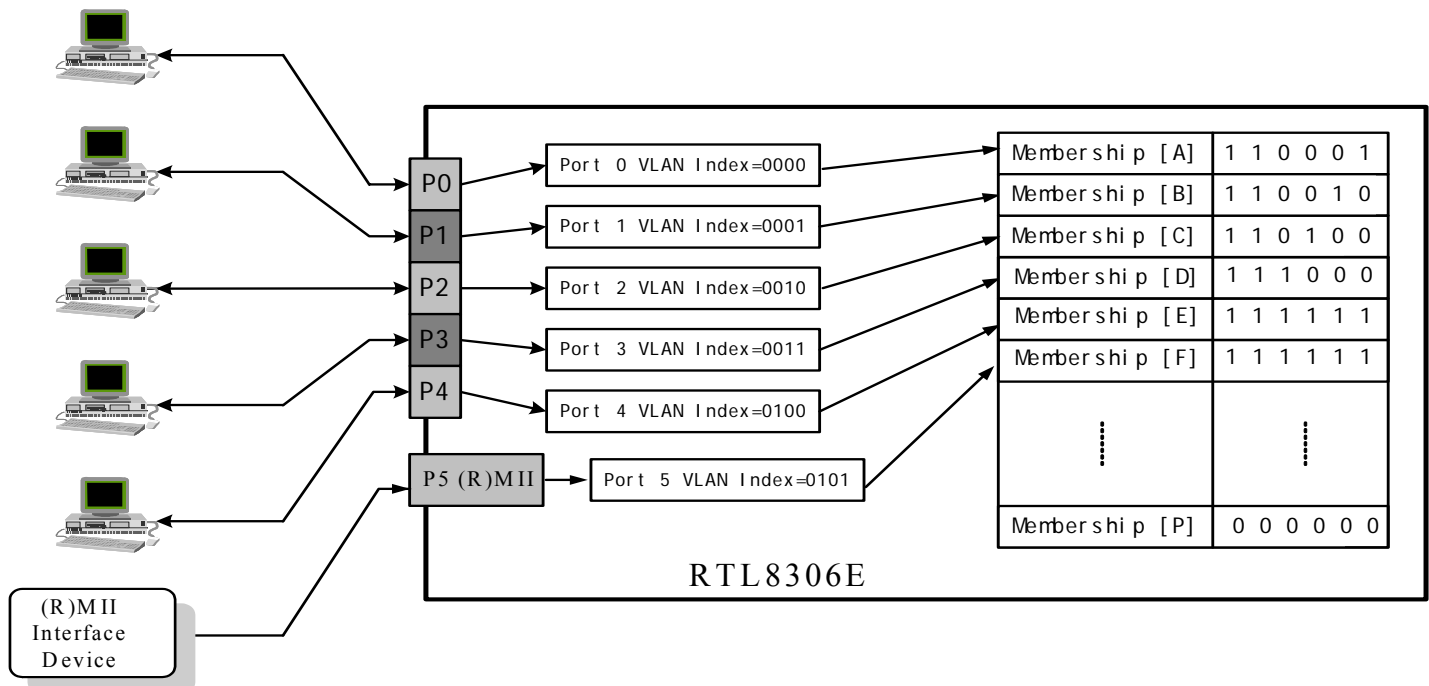
Figure 15. VLAN Grouping with Port5 MAC in Dual-(R)MII Mode
