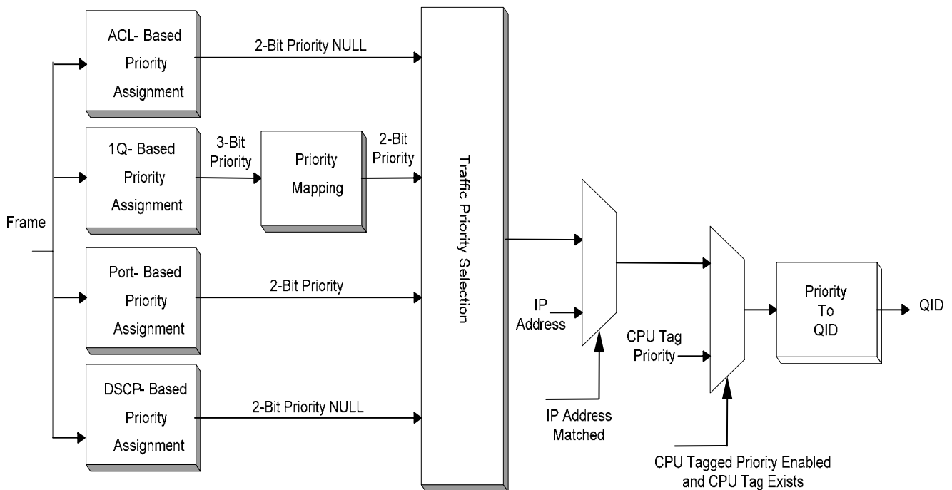
Figure 18. RTL8306E Priority Assignment Diagram
