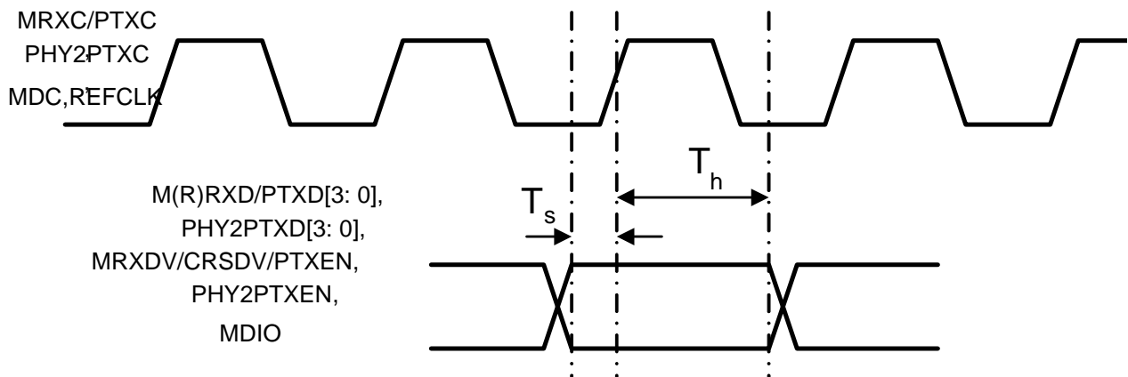
Figure 28. Reception Data Timing of MII/RMII/SMI Interface
