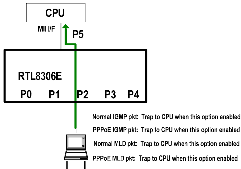
Figure 21. IGMP & MLD Application Example
