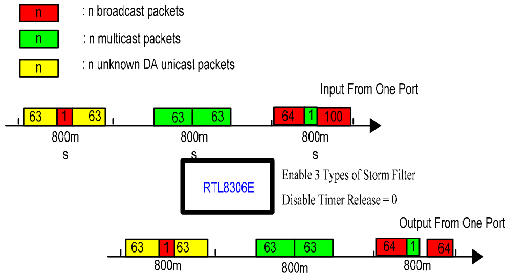
Figure 20. Storm Filter Application Example
