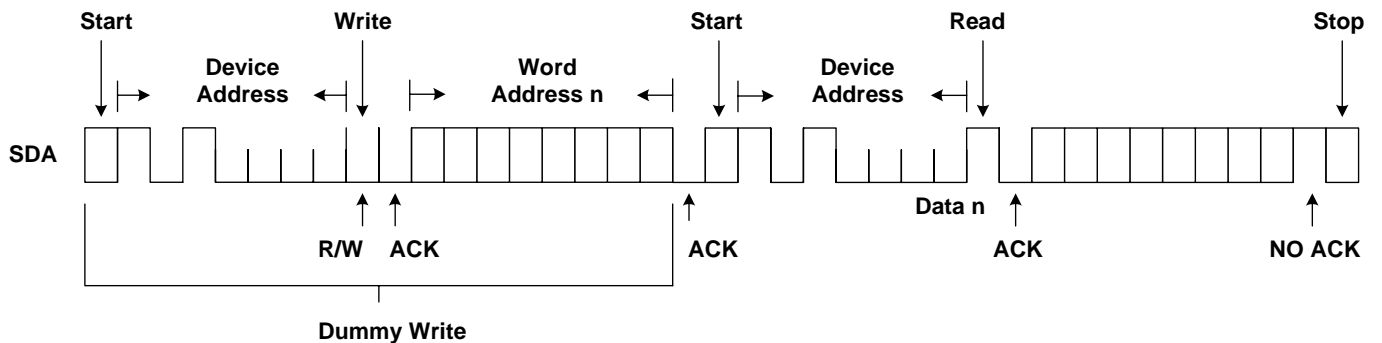
Figure 7. Random Read
