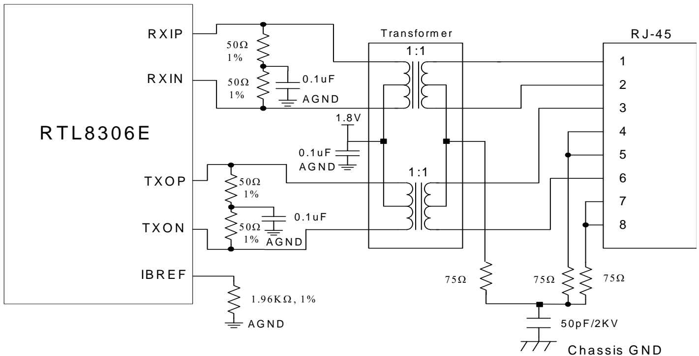
Figure 30. UTP Application for Transformer with Connected Central Tap
