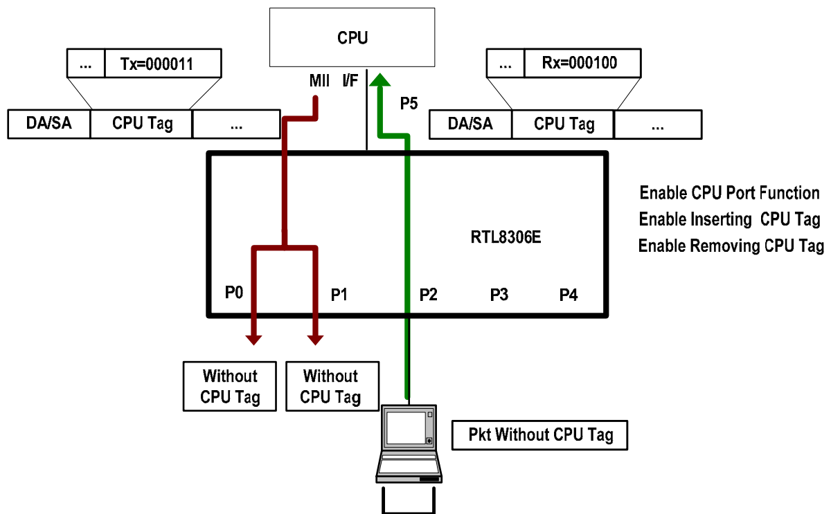
Figure 22. CPU Tag Application Example
