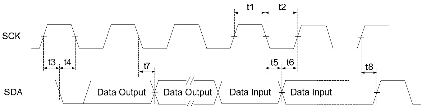
Figure 19. I2C Master Mode Timing
