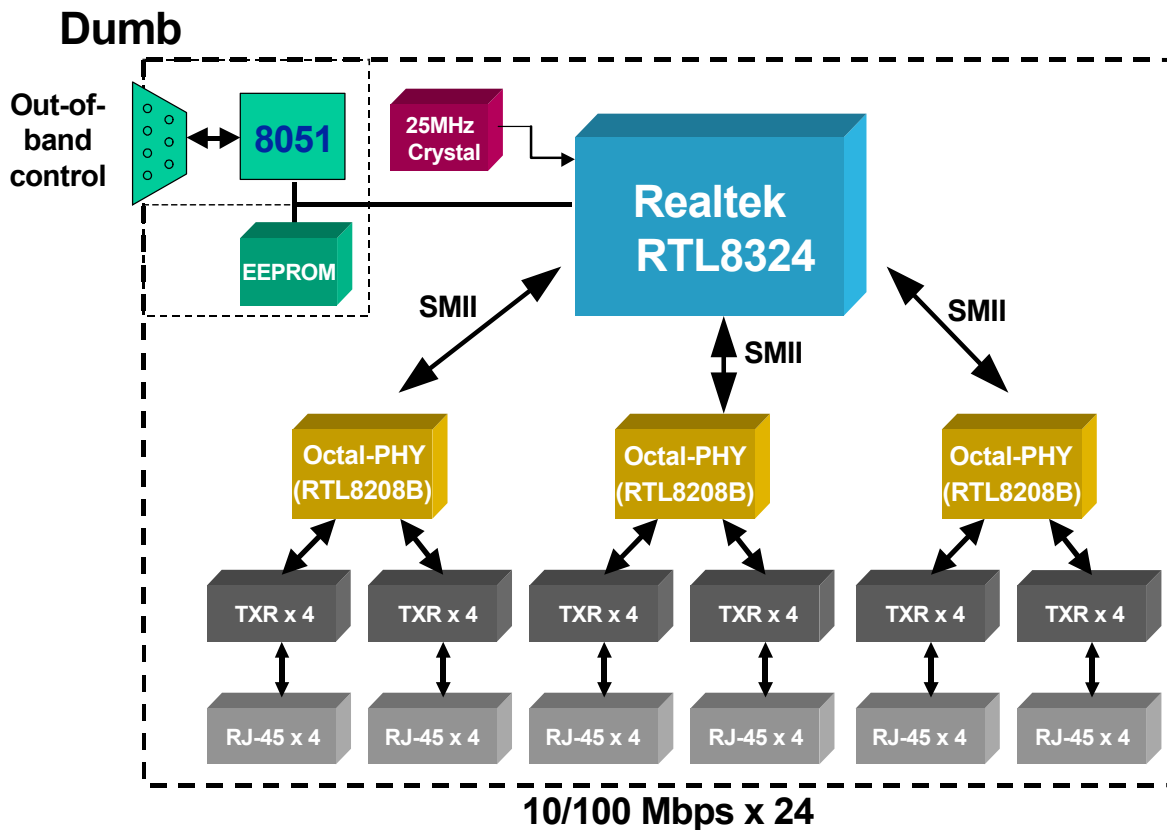
Figure 1. Block Diagram
