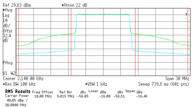
Post - DPD@2140MHz
