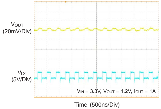
Voltage Ripple
