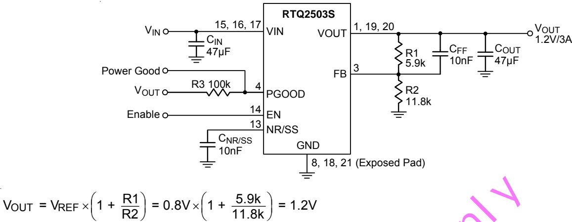
Figure 1. Configuration Circuit for V OUT Adjusted by a Resistive Divider
