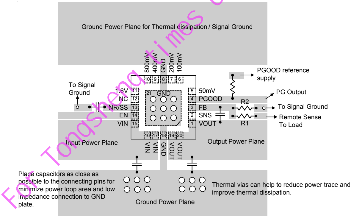
Figure 10. PCB Layout Guide
