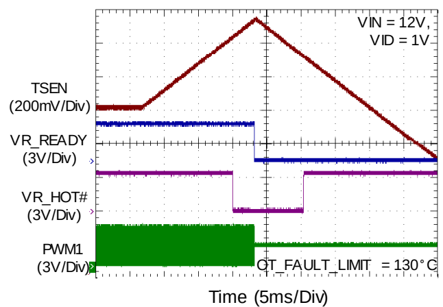
VR OTP
