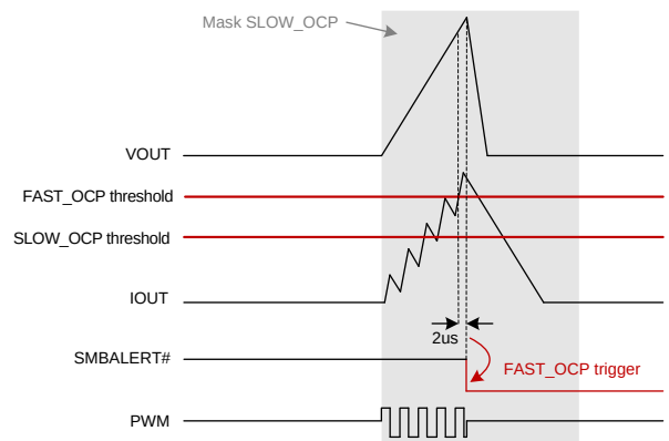
Figure 20. Fast Over-Current Fault
