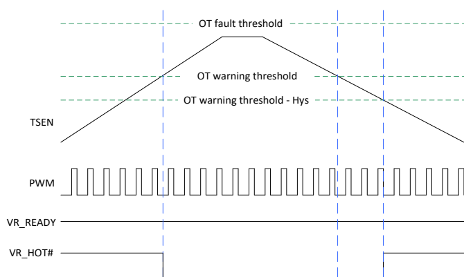
Figure 17. Thermal Warning
