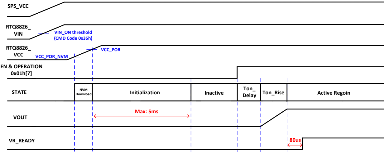
Figure 3. Power-ON Timings
