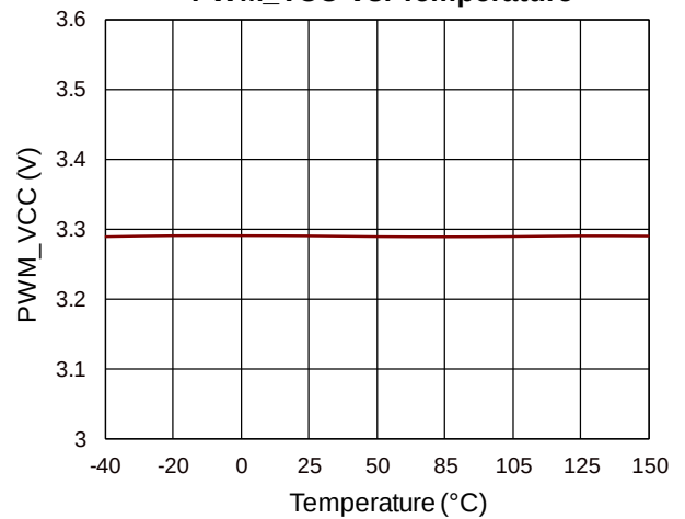
PWM_VCC vs. Temperature
