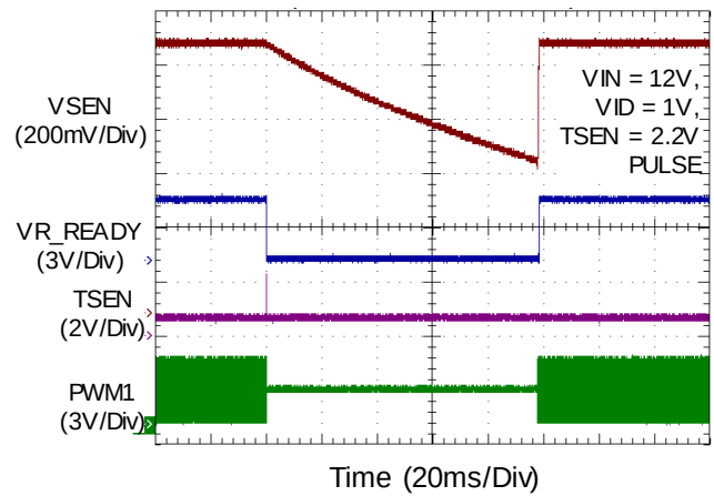
SPS Fault
