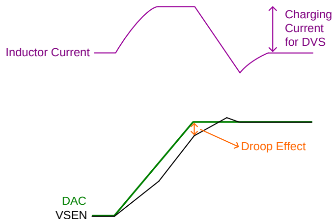
Figure 10. Droop Effect in V_{OUT} Transition
