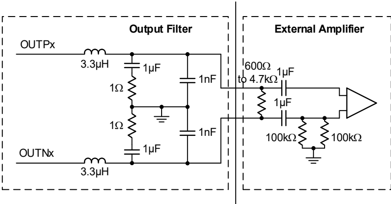
Figure 19. Output Filter
