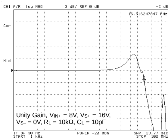
-3dB Bandwidth
