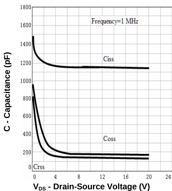
Capacitance
