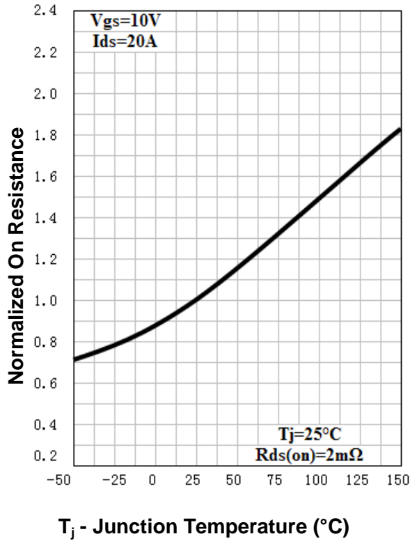
Drain-Source On Resistance
