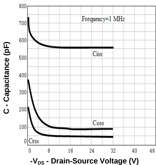
Capacitance
