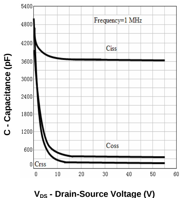
Capacitance
