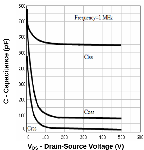
Capacitance
