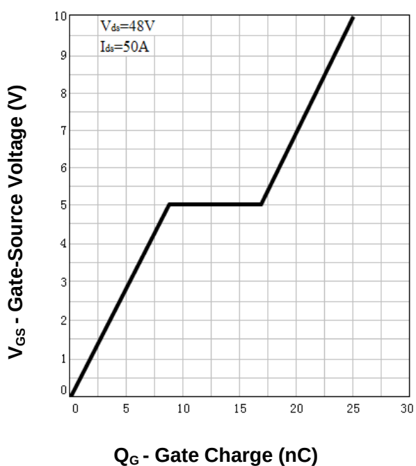
Gate Charge
