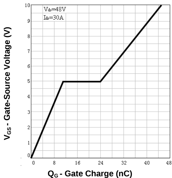
Gate Charge
