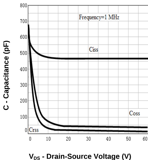
Capacitance
