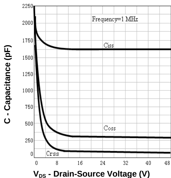
Capacitance
