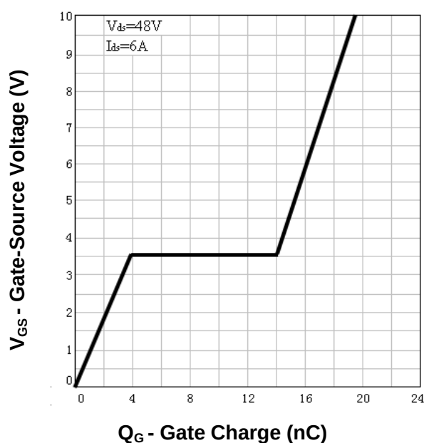
Gate Charge
