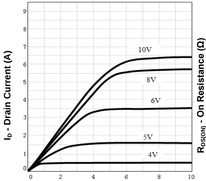
Output Characteristics
