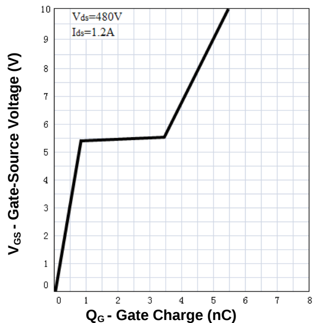
Gate Charge
