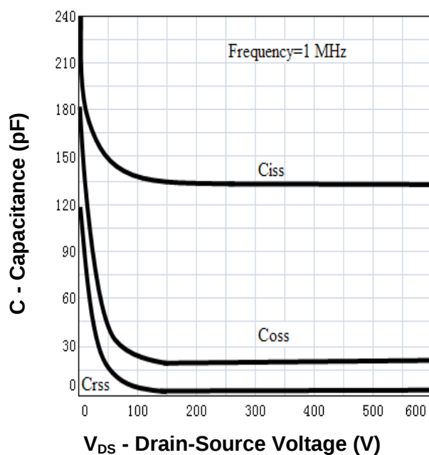
Capacitance
