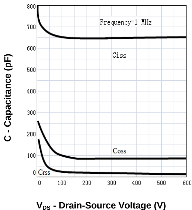
Capacitance
