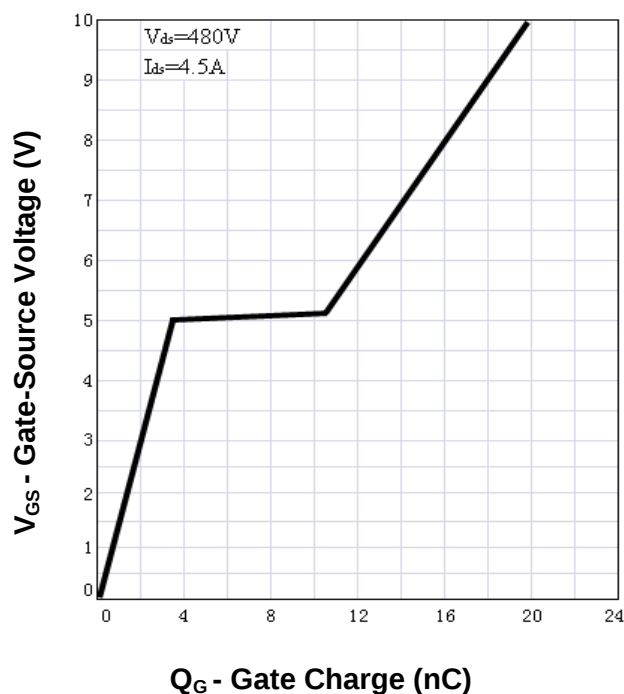
Gate Charge
