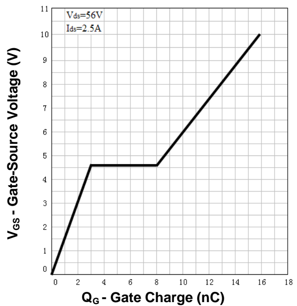
Gate Charge
