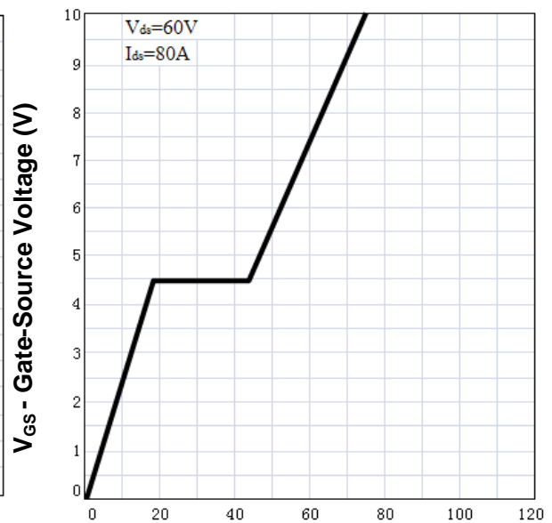
Gate Charge
