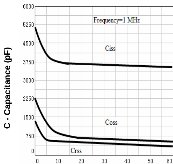
Capacitance
