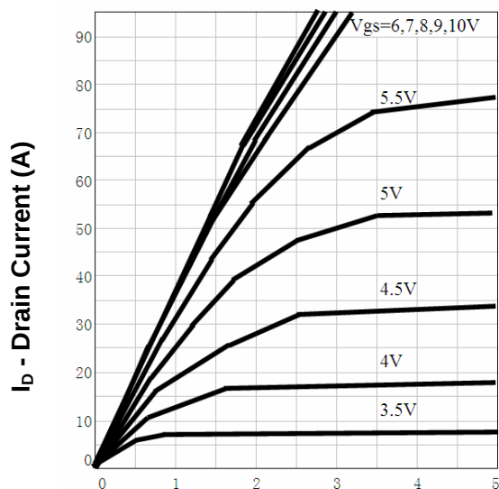
Output Characteristics
