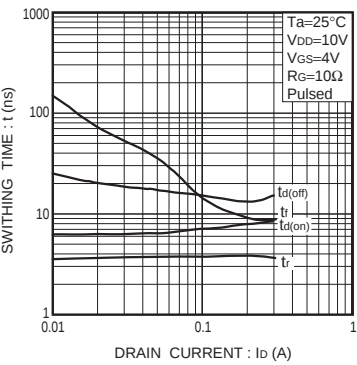
Fig.7 Switching characteristics
