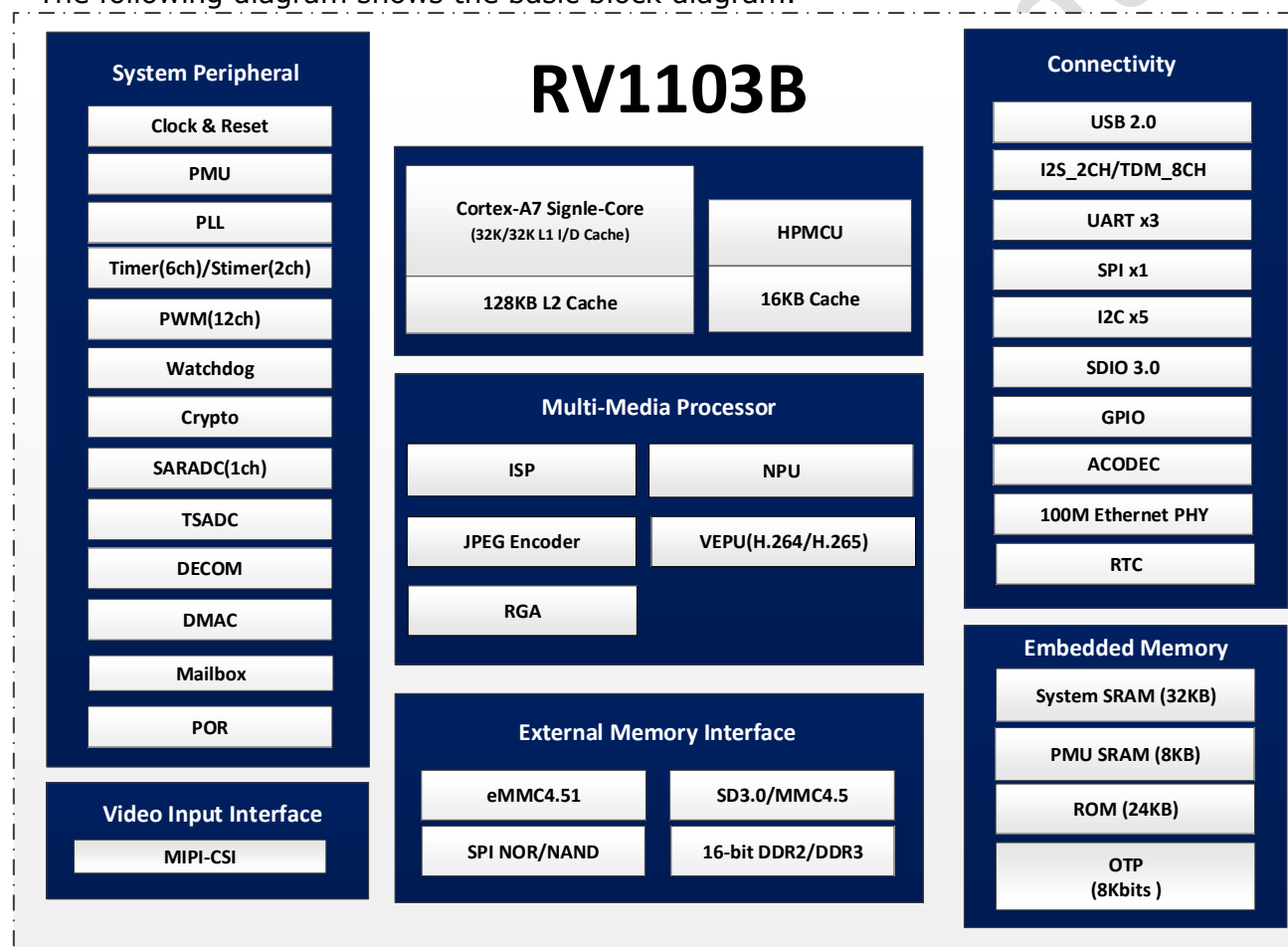
Fig. 1-1 Block Diagram
