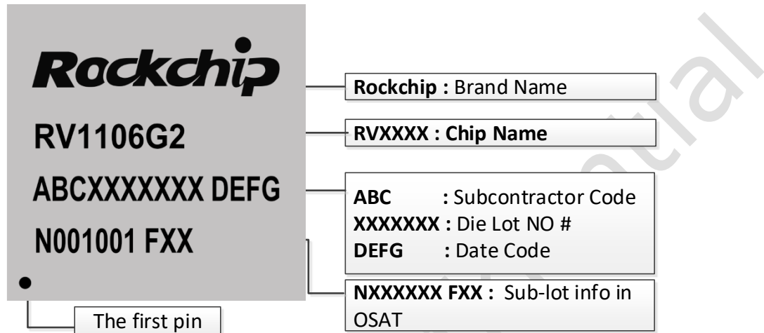
Fig.2-1 Package definition
