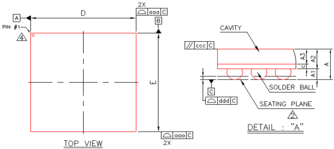
Fig.2-3 Package Top and Side View
