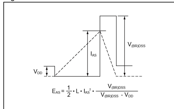
Fig.3-2 Avalanche Waveform
