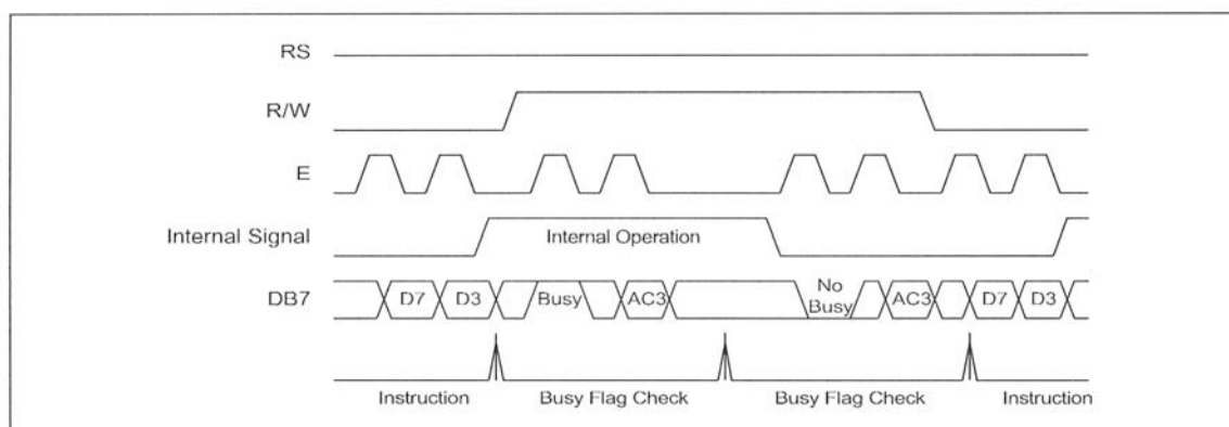
Figure 6. Example of 4-bit Bus Mode Timing Sequence
