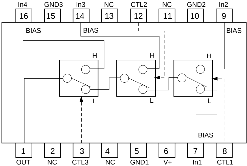
Block diagram
