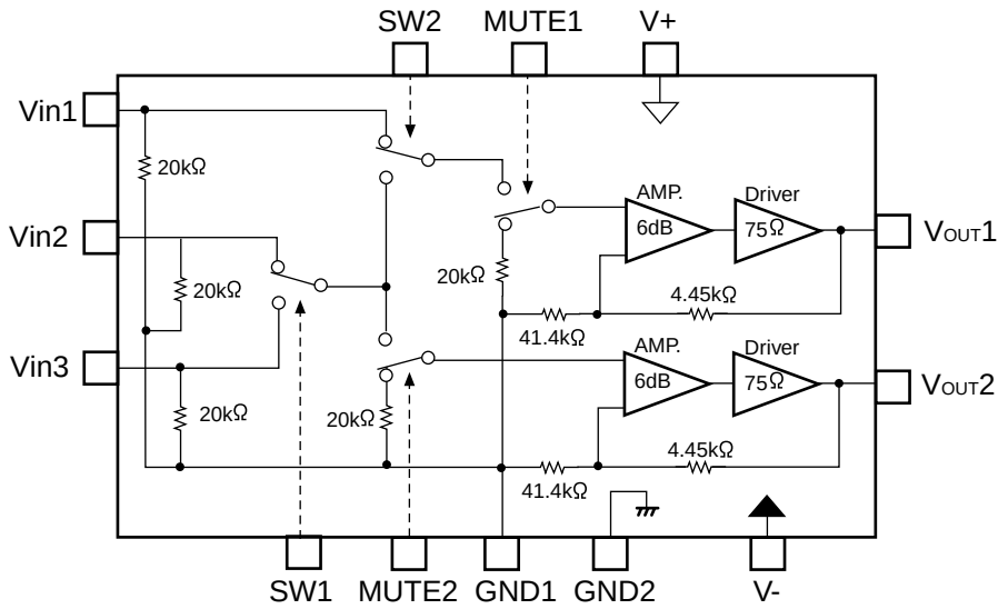
2. Block diagram
