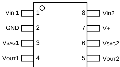
1. Pin layout
