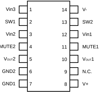
1. Pin layout
