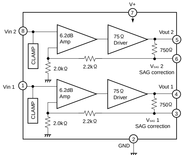
2. Block diagram
