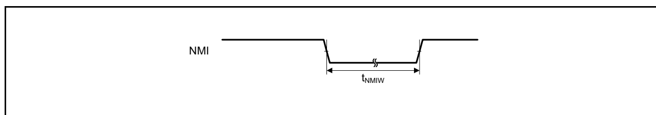
Figure 5.39 NMI Interrupt Input Timing
