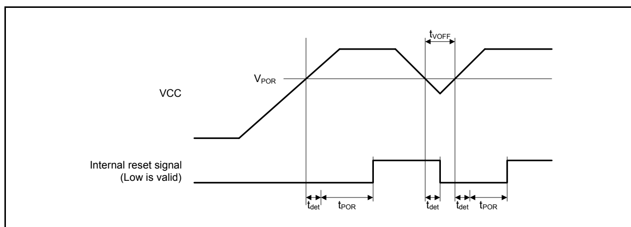
Figure 5.79 Power-on Reset Timing
