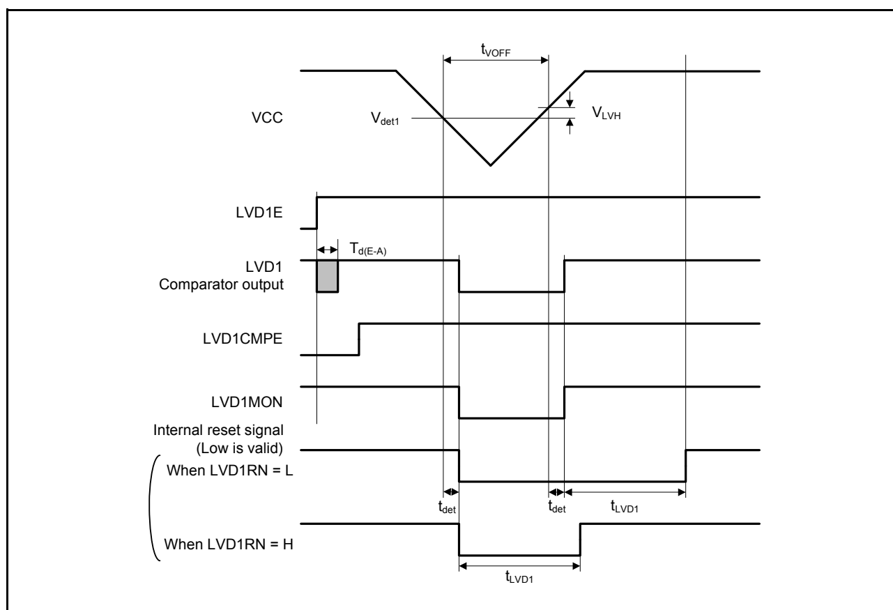
Figure 5.81 Voltage Detection Circuit Timing (V det1 )
