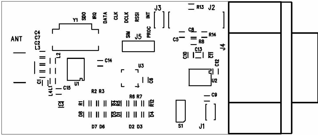
Silkscreen
