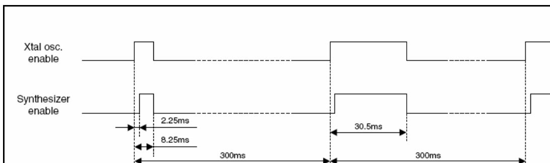
Figure 4. Duty Cycle Mode Wake-up Timing
