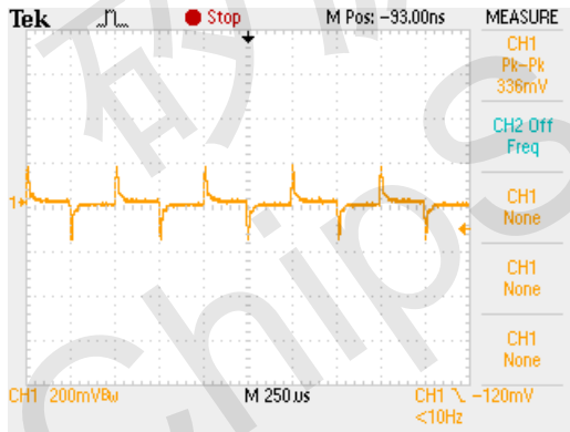
LOAD TRANSIENT RESPONSE (V IN =5V, V OUT =3.3V, I OUT =500-1500mA, 1A/μS)
