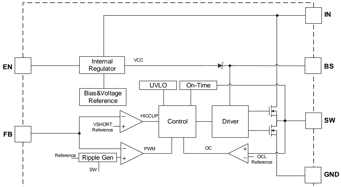
Block Diagram
