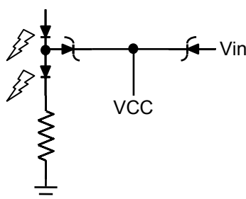
Figure 2. Bootstrapping Circuit
