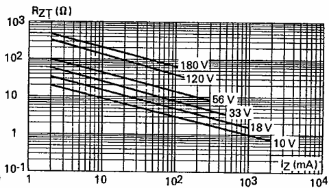
Fig. 4 - Differential resistance R_{ZT} versus I_Z (maximum values).
