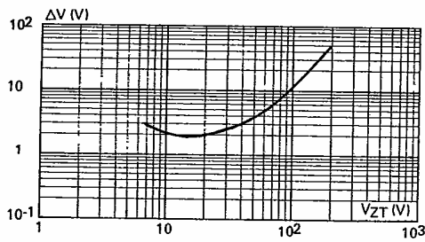
Fig. 5 - Regulation voltage variation for I_Z variation between 10 % and 50 % of I_{ZM} (typical values) D.C. measure ( T_{case} = 25^\circ C ).
