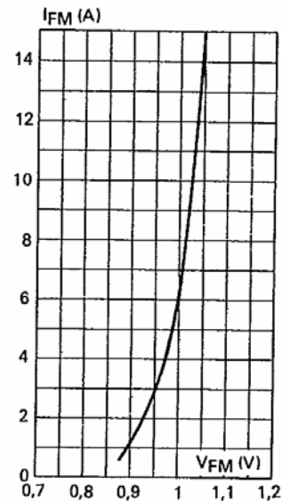
Fig. 9 - Peak forward current I_{FM} versus peak forward voltage drop V_{FM} at T_{\text{case}} = 25^{\circ}\text{C} (typical values).
