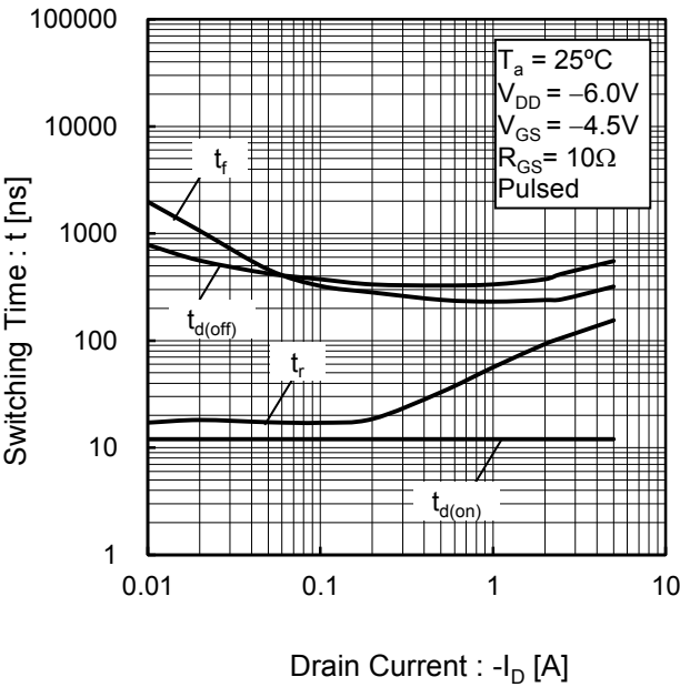
Fig.20 Switching Characteristics
