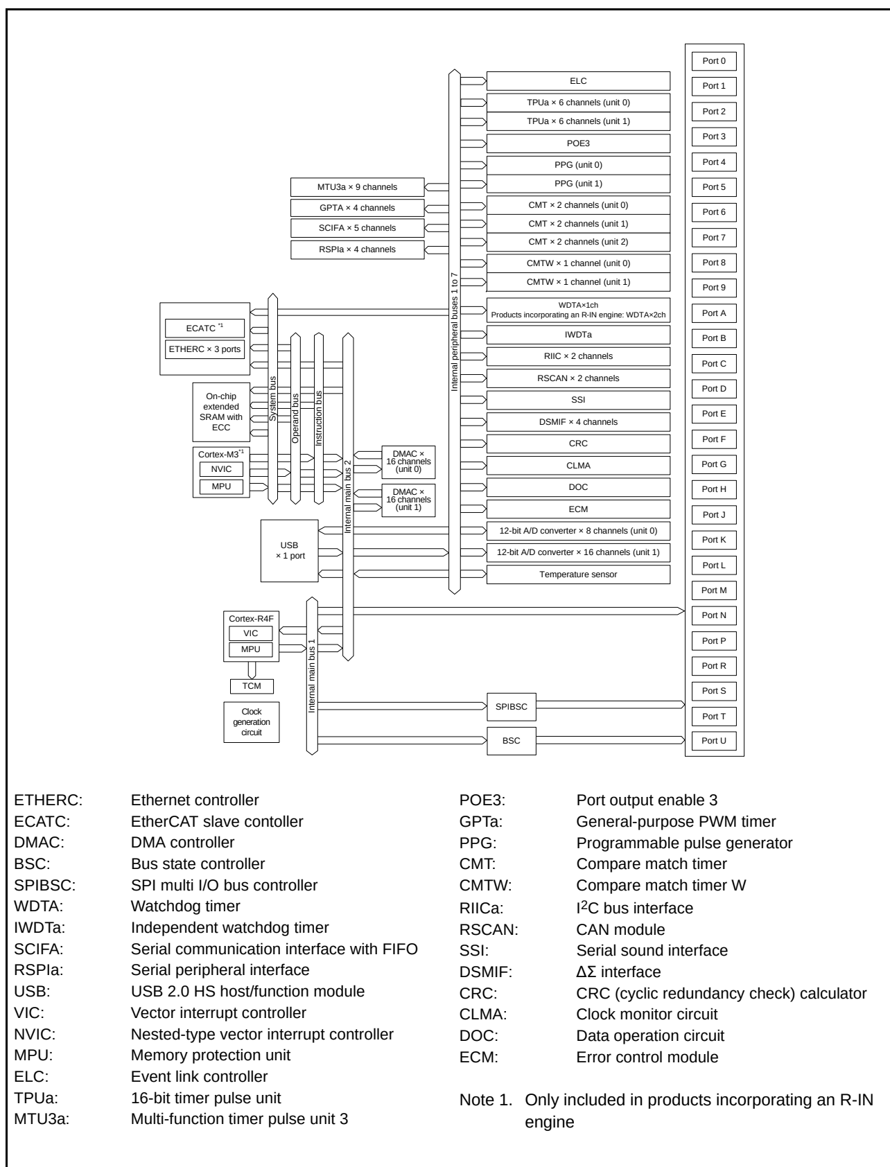
Figure 1.1 Block Diagram
